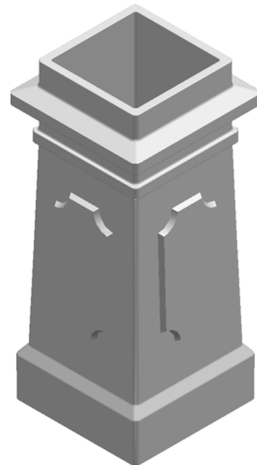
ISOMETRIC VIEW 1:10
