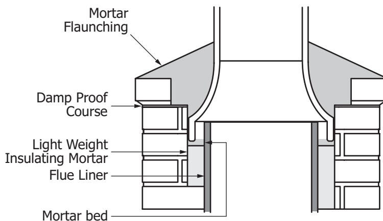
Flaunching
