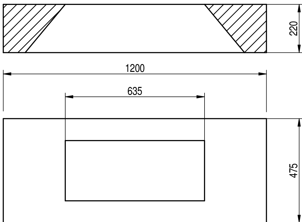
BOTTOM VIEW
